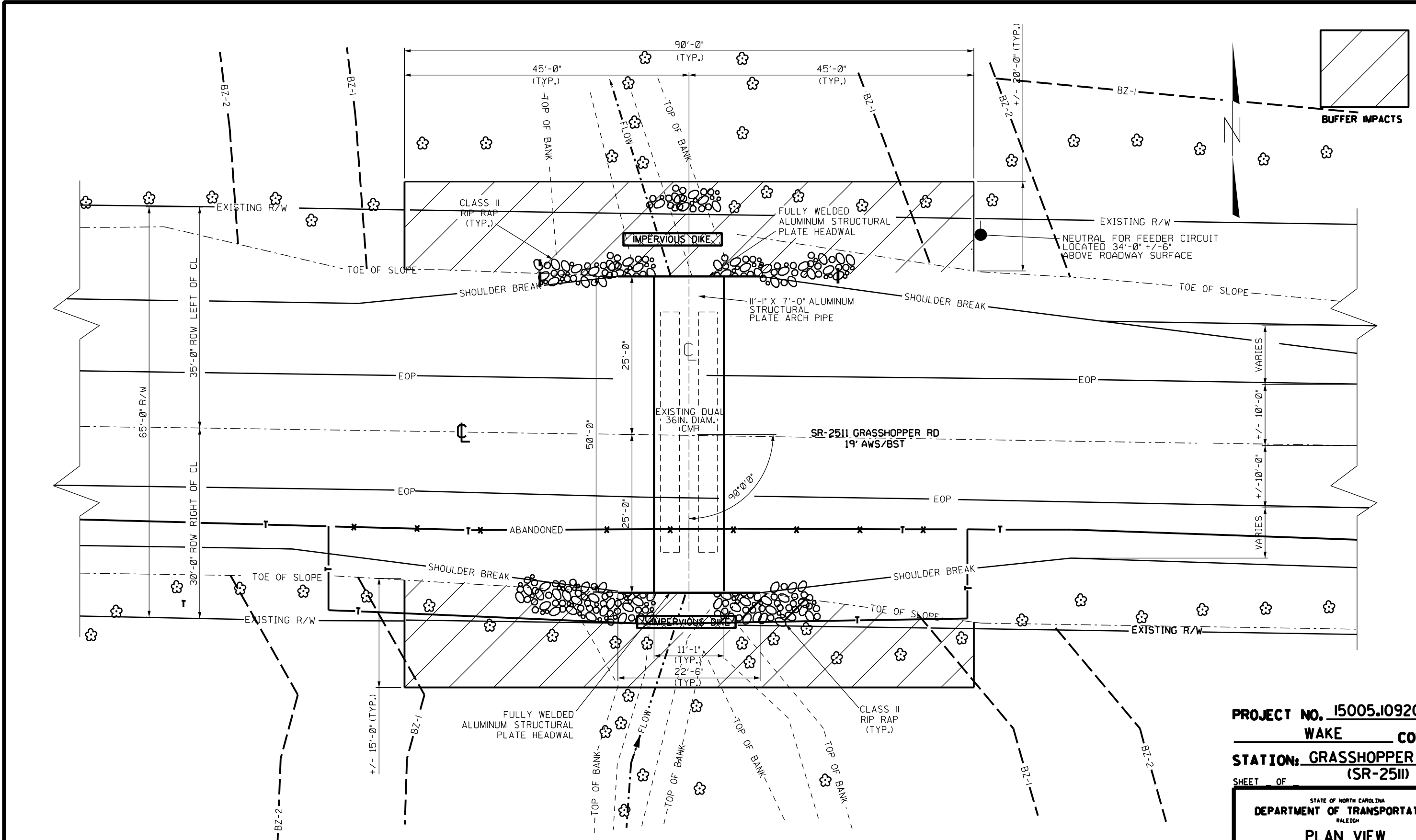
PLAN VIEW 11'-1" X 7'-0" CORRUGATED ALUMINUM STRUCTURAL PLATE ARCH
